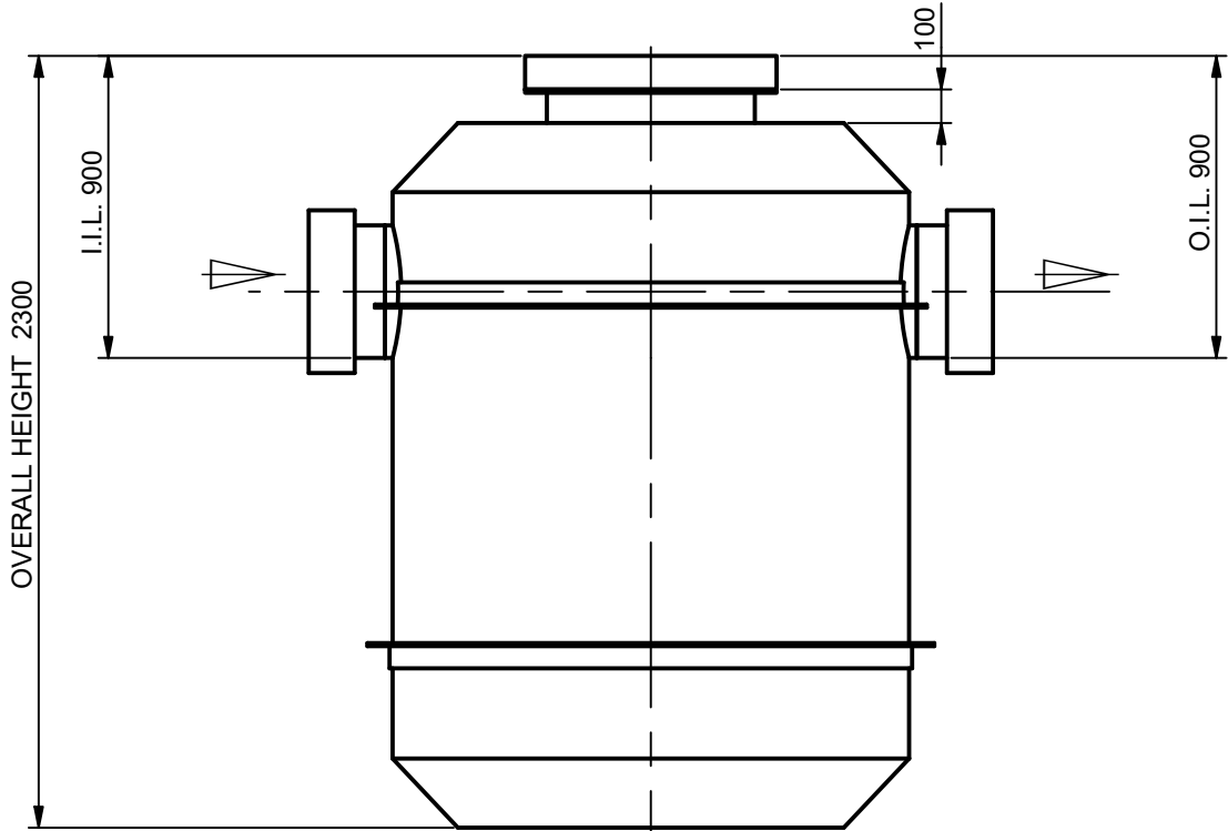
ELEVATION VIEW
